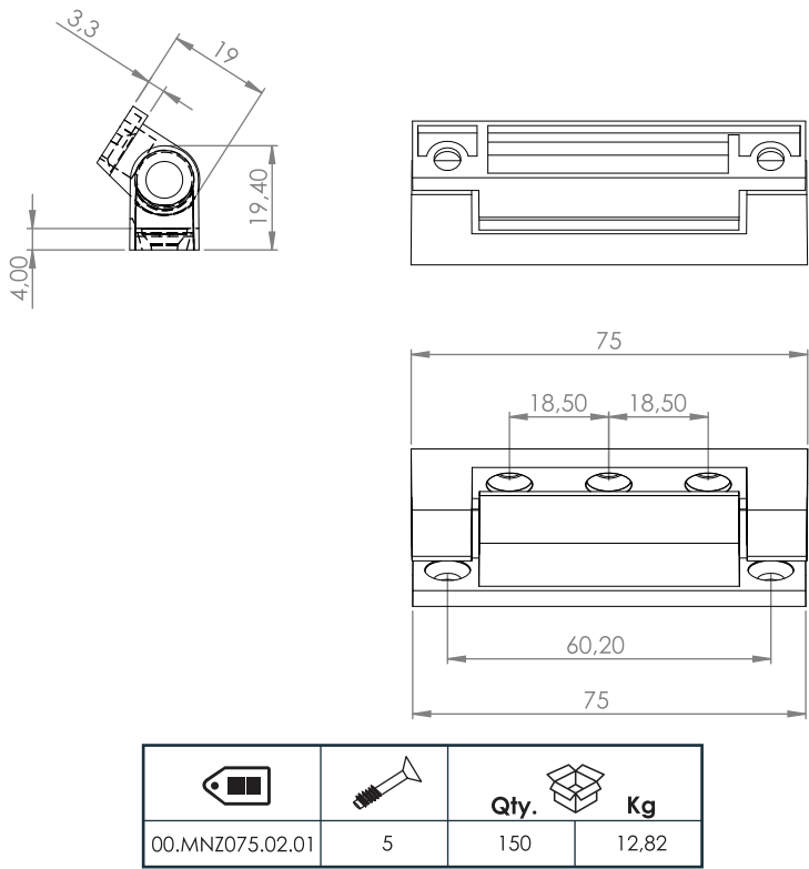
● Zinc Window Hinge 75 mm
