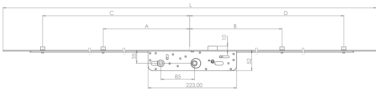
PZ: 85 mm Backset: 35 mm - Balcony (Akpen Series - Metal Lock Case)
