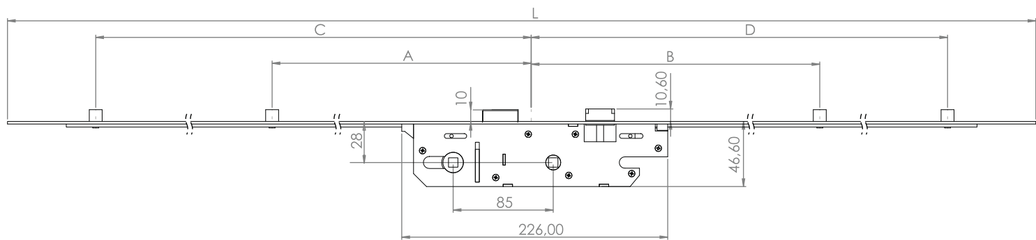
PZ: 85 mm Backset: 28 mm - Balcony (Plastic Lock Case) ●
