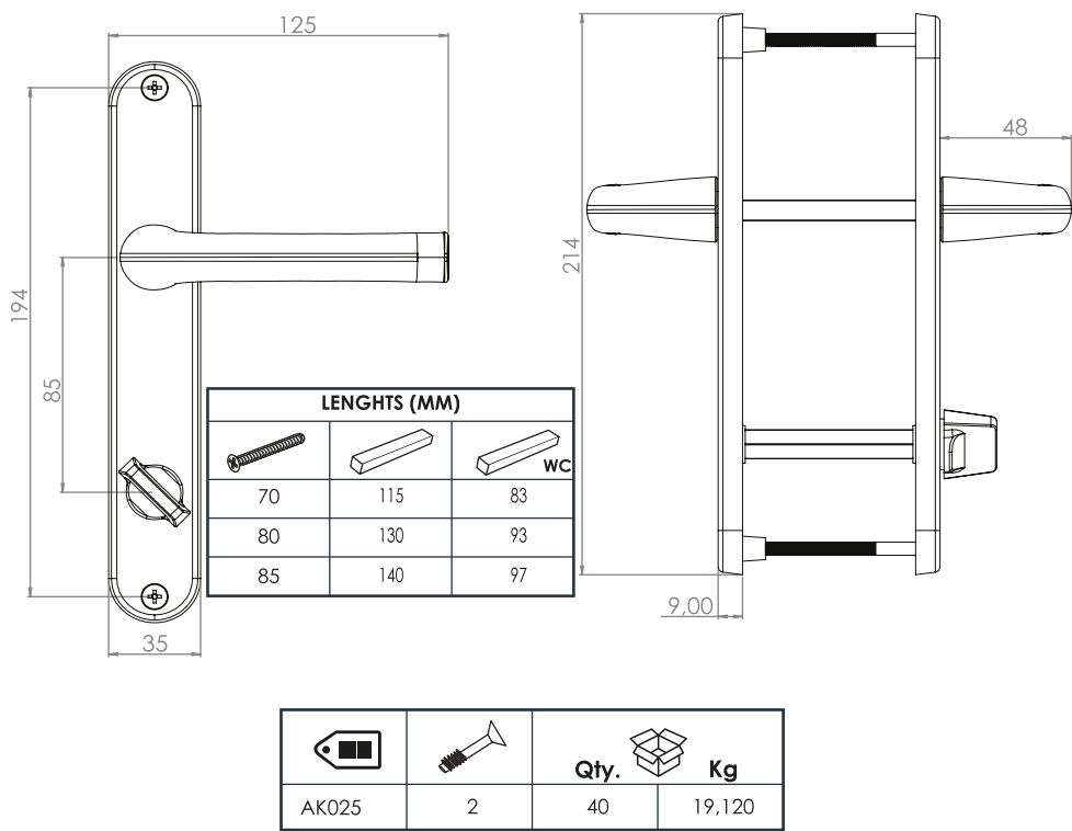
Mega Aluminium Balcony Handle ● PZ: 85 mm Backset: 35 mm
