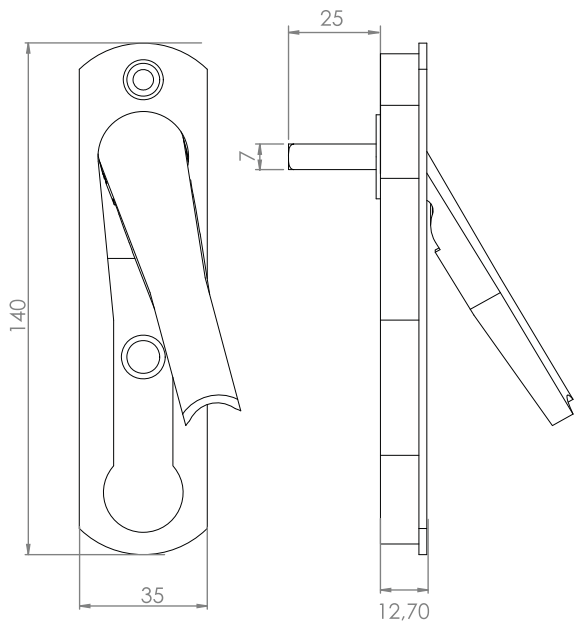
● Pop-Up Handle Zinc
