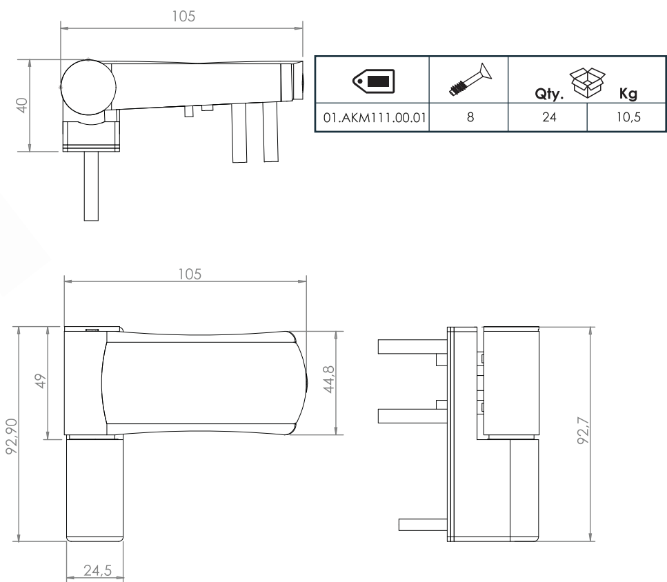
● Aluminium 3D Adjustable Door Hinge
