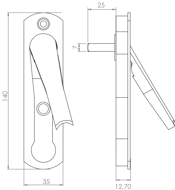
Pop-Up Handle Aluminium ●
