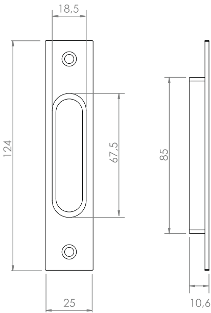
● Sliding Handle (POOL) Inlaid Small
