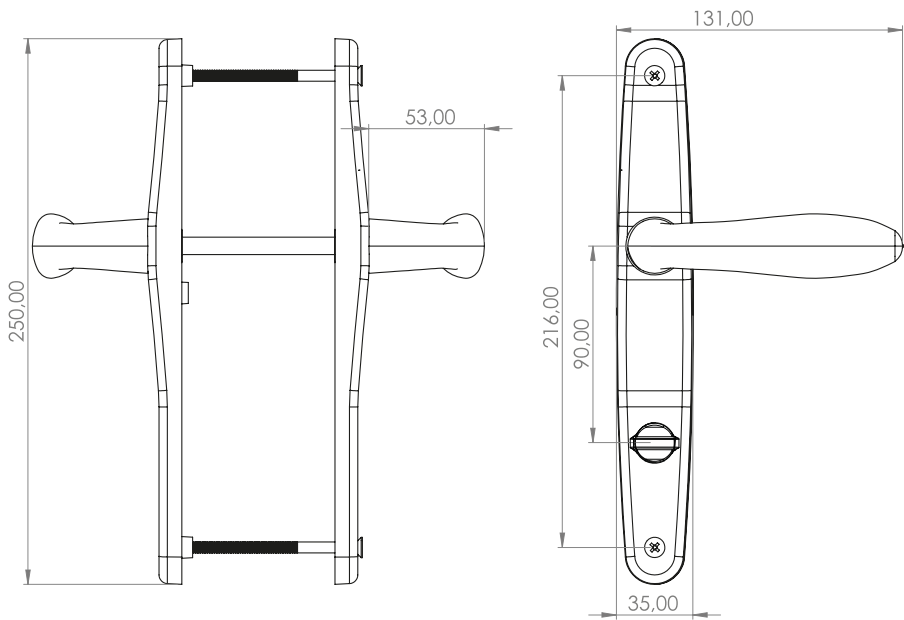
● Ada Aluminium WC Handle PZ: 90 mm Backset: 35 mm
