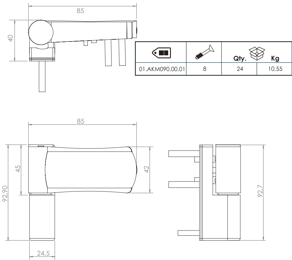
Junior Zinc 3D Adjustable Door Hinge ●
