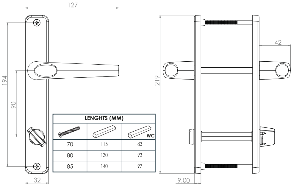
● Bosna Aluminium WC Handle PZ: 90 mm Backset: 32 mm
