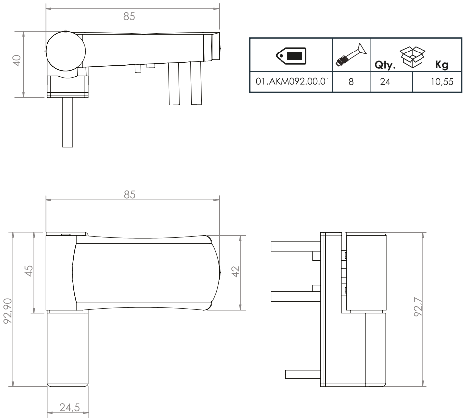
Junior Aluminium 3D Adjustable Door Hinge ●
