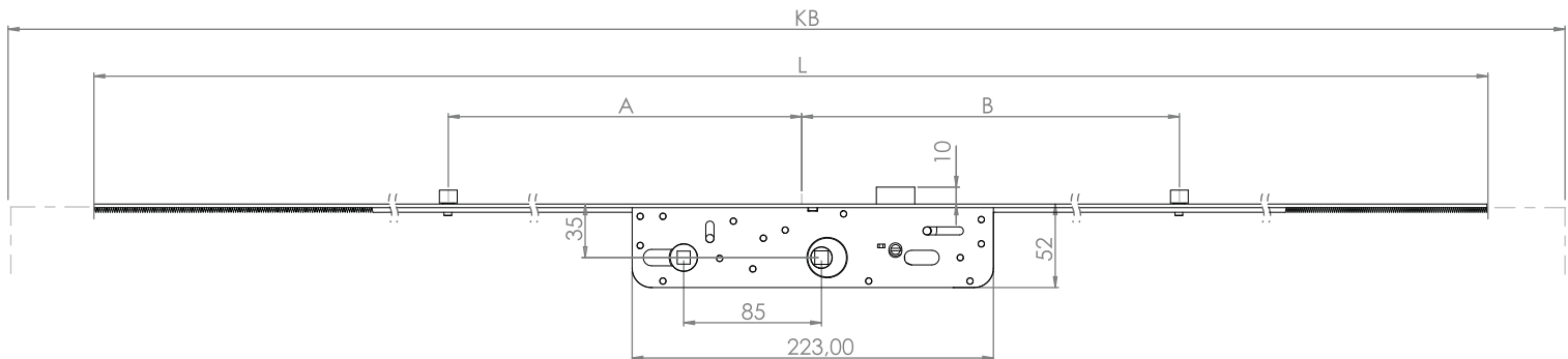
PZ: 85 mm Backset: 35 mm Cuttable (Metal Lock Case)
