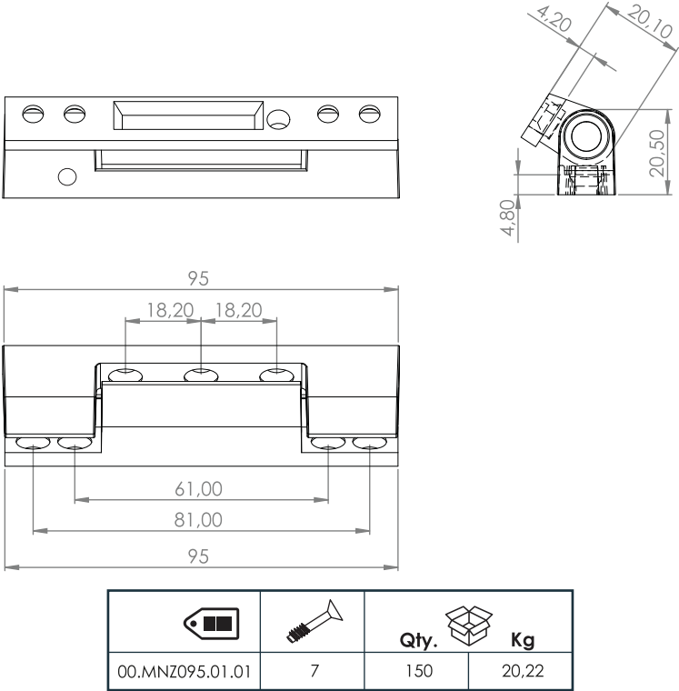
● Zinc Door Hinge 95 mm Outward Opening
