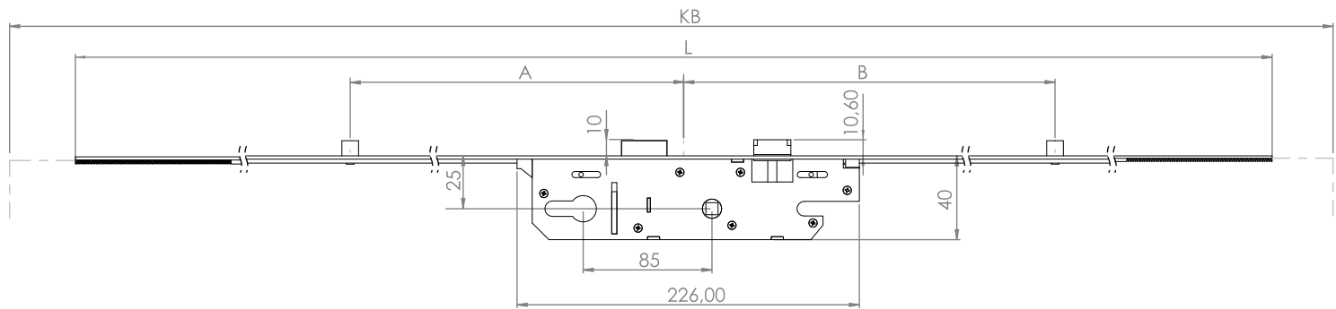
PZ: 85 mm Backset: 25 mm Cuttable (Plastic Lock Case)
