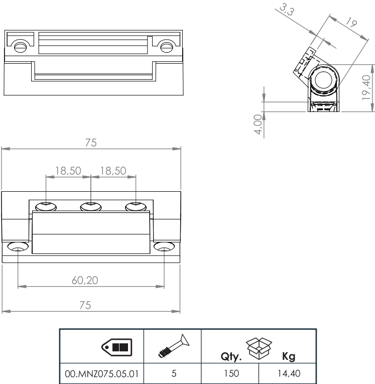
● Zinc Window Hinge 75 mm For Egepen Max / Adopen Atlantik
