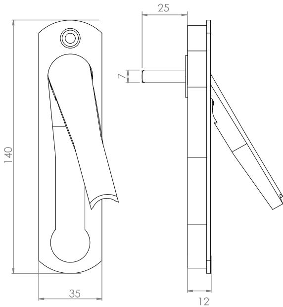
Pop-Up Handle Plastic ●
