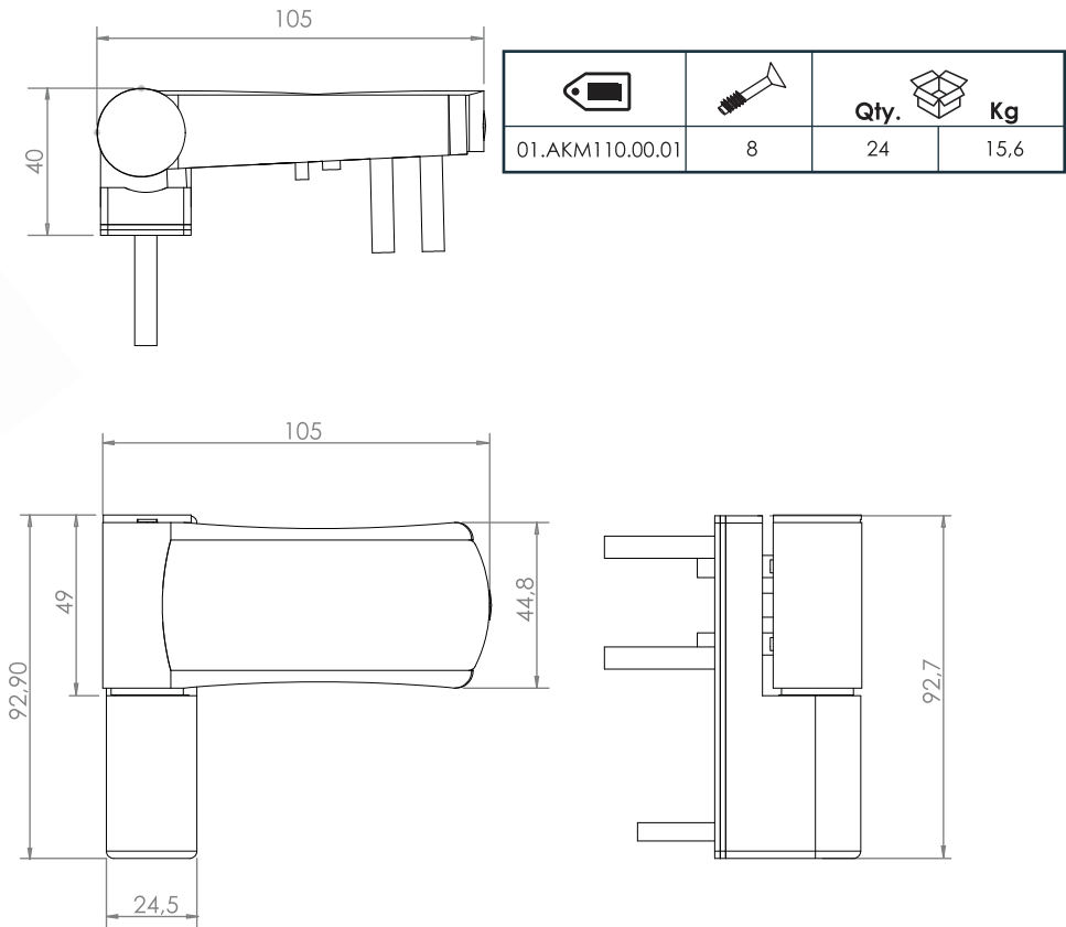
● Zinc 3D Adjustable Door Hinge
