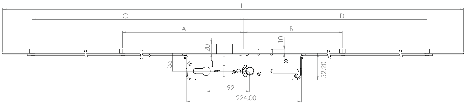
PZ: 92 mm Backset: 35 mm (Deluxe Series - Metal Lock Case) ●
