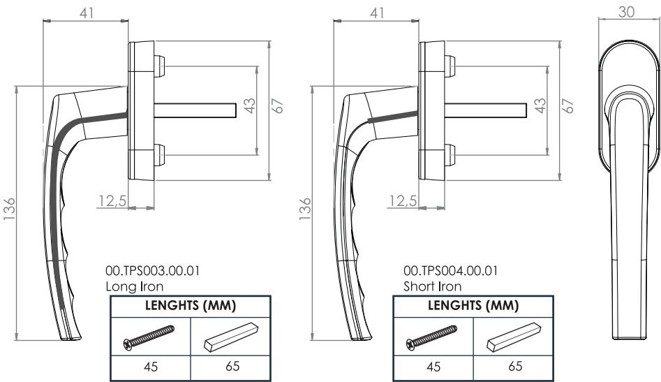
Plastic Window Handle ●
