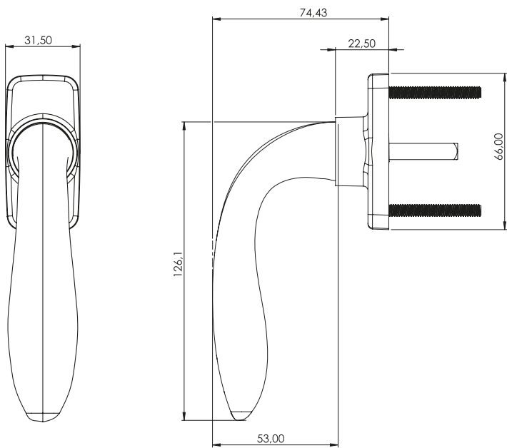
● Ada Aluminium Window Handle
