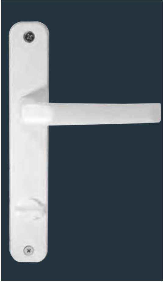
Pinar Aluminium WC Handle ● PZ: 90 mm Backset: 32 mm
