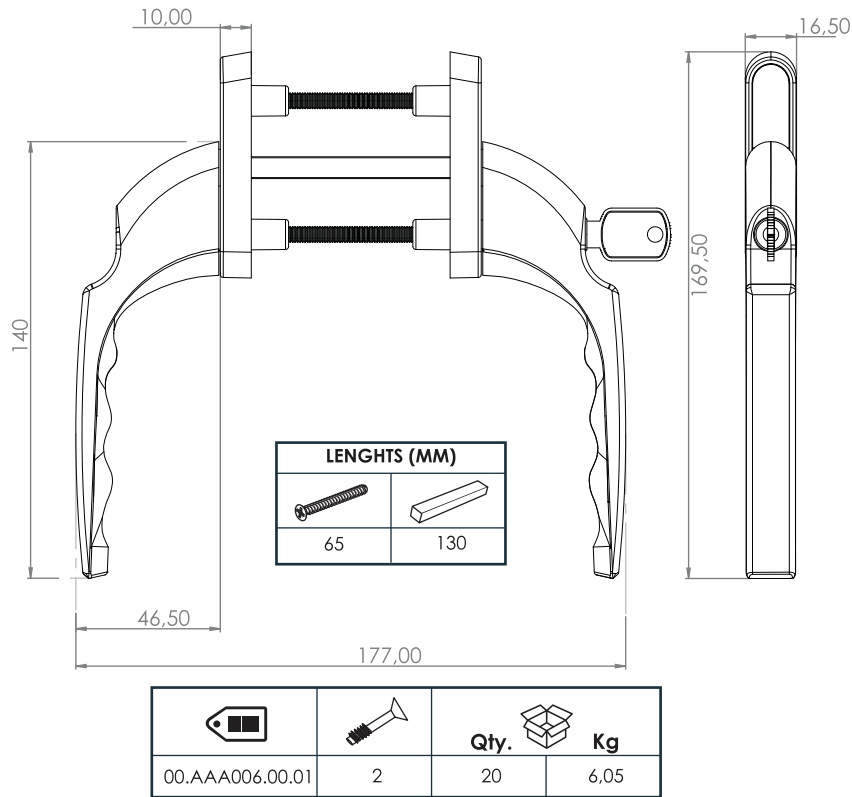
● Lockable Double Side Outward Opening Handle
