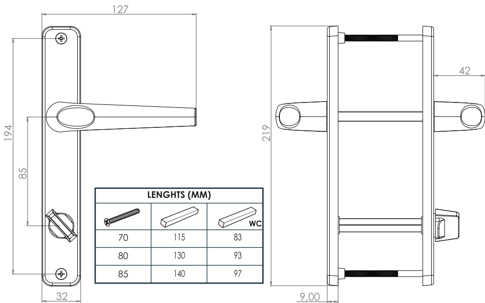
● Bosna Aluminium Balcony Handle PZ: 85 mm Backset: 32 mm
