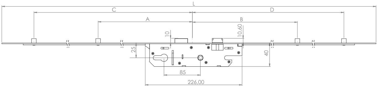
PZ: 85 mm Backset: 25 mm (Plastic Lock Case) ●
